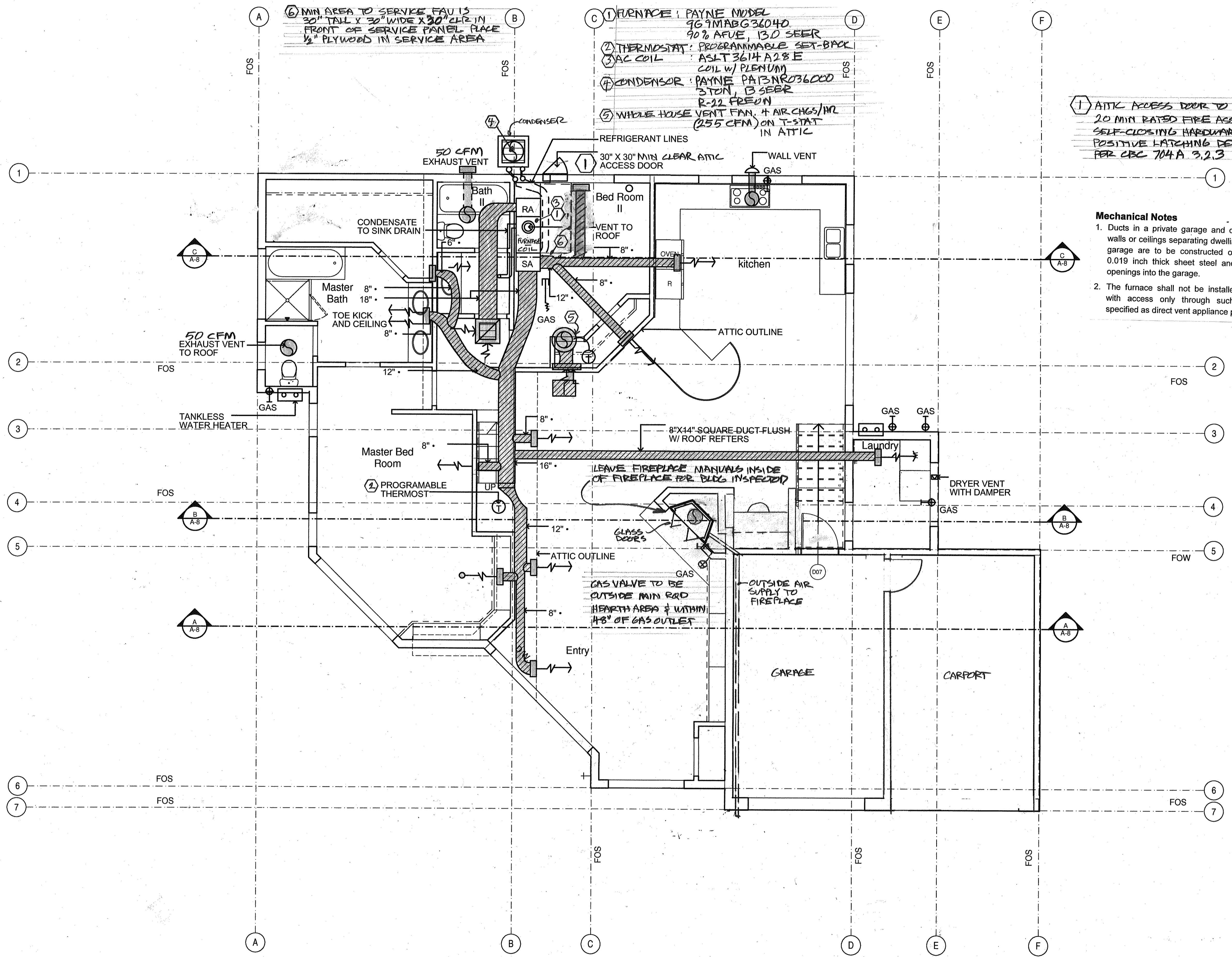
1 GROUND FLOOR MECHANICAL PLAN SCALE: 1/4" = 1'-0"
