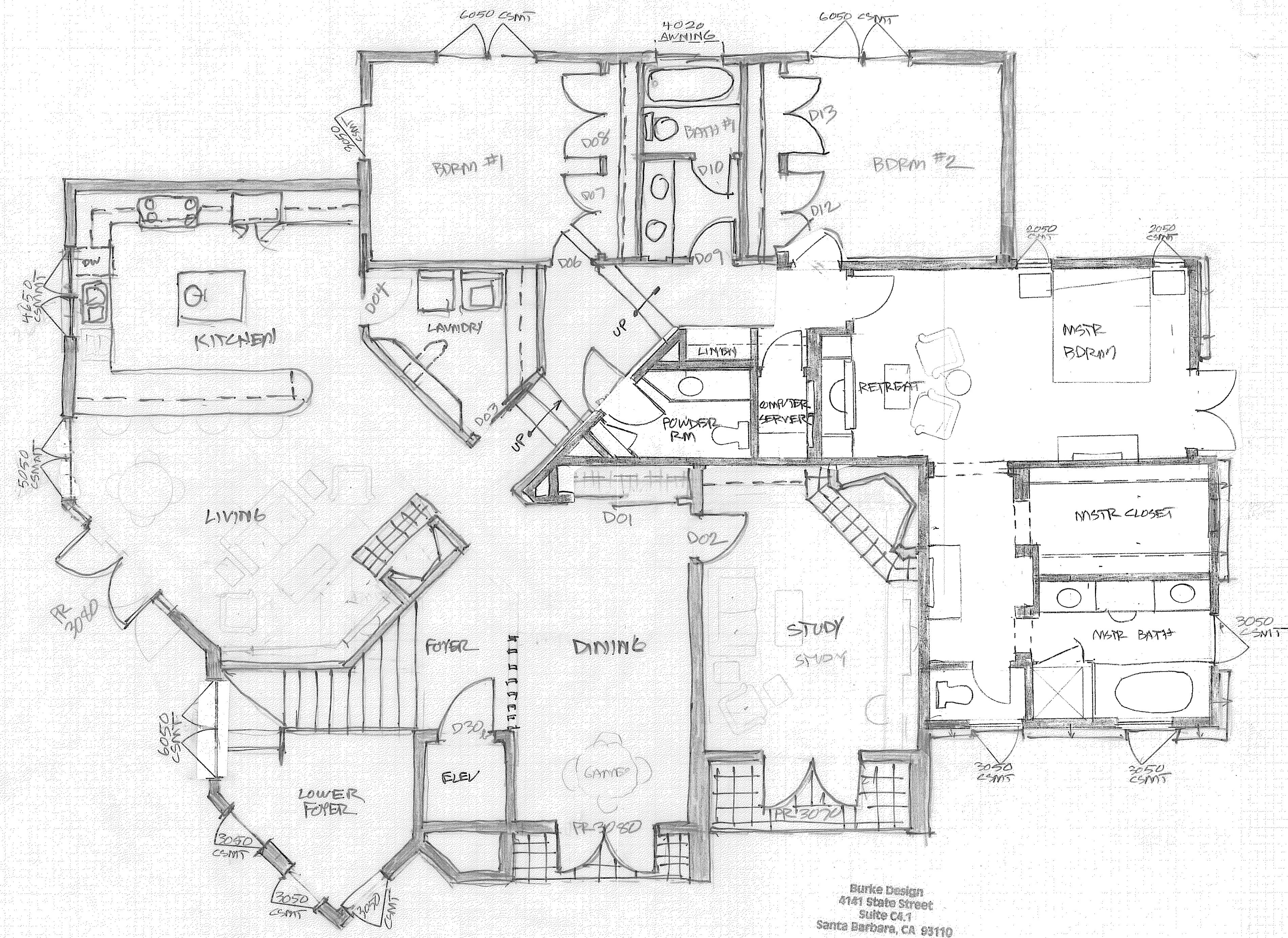
FLOOR PLAN SCALE 1/4"
